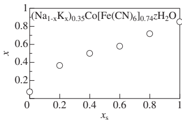
FIG. 1. Relation between K^+ concentration ( x ) in (Na_{1-x}K_x)_{0.35}Co[Fe(CN)_6]_{0.74z}H_2O films and that ( x_s \equiv \frac{[K]}{[K]+[Na]} ) in dipping solution.
