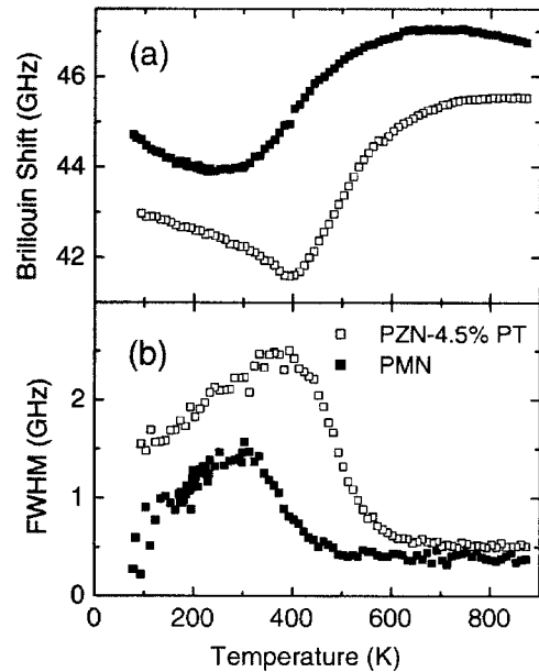
FIG. 2. Brillouin shift (a) and FWHM (b) of PMN and PZN-4.5%PT as a function of temperature.
