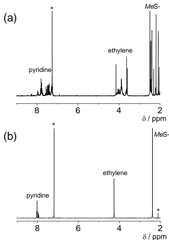
Figure 1. ^1\text{H} NMR spectra of (a) 2 and (b) [\mathbf{2}\cdot\text{Ca}]\text{Cl}_2 (400 MHz, \text{CDCl}_3 , 298 K). Peaks marked with an asterisk * are due to solvent impurities.
