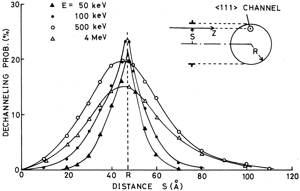
FIG. 2. Calculated (111) dechanneling probabilities of helium ions for a channel at distance s from the center of the vacancy dislocation loop in aluminum. The Burgers vector is \frac{1}{3}a\langle 111 \rangle , parallel to the channel, and it is perpendicular to the plane of the loop. The same results are expected when the dislocation loop is an interstitial one.
