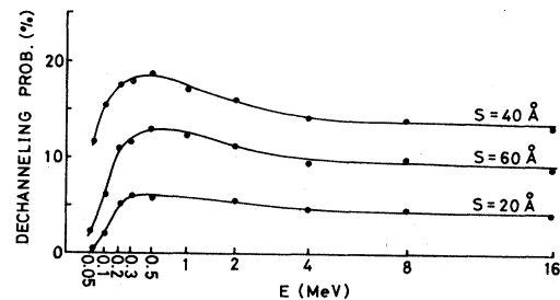
FIG. 5. Calculated energy dependence of \langle 111 \rangle dechanneling probabilities of helium ions for channels at various s , the distance from the center of the dislocation loop in aluminum.
