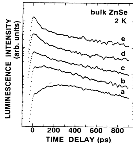
FIG. 5. Time-resolved luminescence of the biexciton in bulk ZnSe at 2 K under excitation-energy densities of a , 0.9; b , 6.3; c , 15; d , 84; and e , 188 \mu\text{J}/\text{cm}^2 . The luminescence intensity is plotted on a logarithmic scale.
