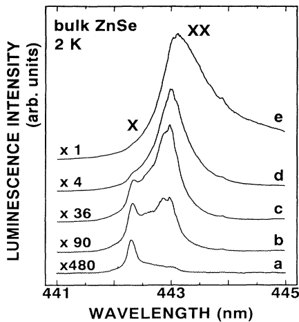
FIG. 4. Time-integrated luminescence spectra at 2 K taken from bulk ZnSe under excitation-energy densities of a , 0.1; b , 0.6; c , 1.5; d , 6.2; and e , 52 \mu\text{J}/\text{cm}^2 . These spectra are shown after being multiplied by the number that is indicated on the left-hand side of each spectrum for clarity.
