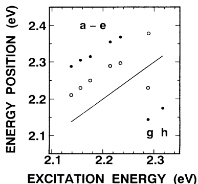
FIG. 2. Excitation energy dependence of the energy positions of antiholes ( \circ ) and satellite holes ( \bullet ). The five data from the left-hand side are taken from spectra (a)–(e) and the others are from (g) and (h) in Fig. 1.
