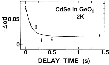
FIG. 6. The temporal change in the depth of spectral holes in CdSe nanocrystals embedded in GeO 2 glass at 2 K. The experimental conditions were the same as those of Fig. 5.
