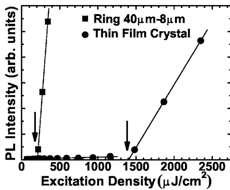
FIG. 4. Excitation density dependence of the highest emission peak intensities of a microring laser (solid square) and a thin film crystal (solid circle). The diameter of a microring laser is 40 \mu\text{m} and the ring width is 8 \mu\text{m} . The thresholds for the laser oscillation of a microring and a thin film crystal are 200 and 1400 \mu\text{J}/\text{cm}^2 , respectively.
