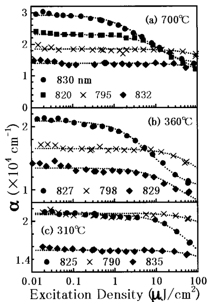
FIG. 2. Excitation density dependence of the optical absorption coefficient in (a) 700 °C, (b) 360 °C, and (c) 310 °C-grown MQWs measured at various wavelengths. Dashed curves are semiempirical saturation fits to the data.
