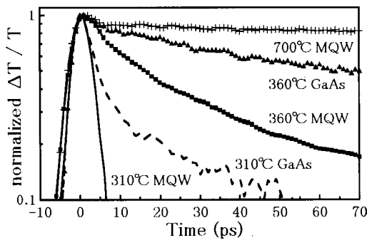
FIG. 3. Normalized temporal changes of differential transmission. The profile for the 310 °C-grown MQW shows the time resolution in this experiment.
