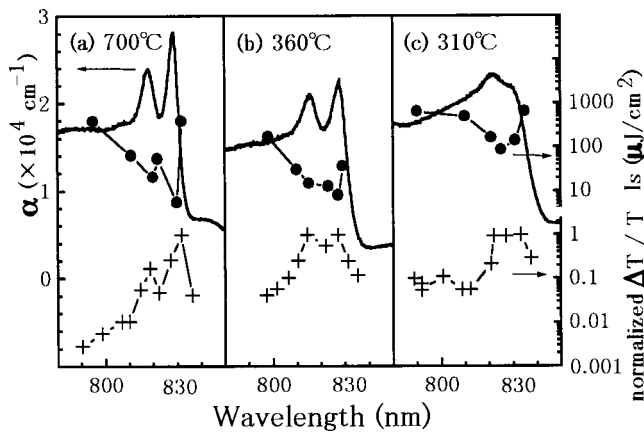
FIG. 1. Absorption spectra ( \alpha , solid lines), saturation densities ( I_s , circles), and the magnitude of the differential transmission at time zero in the pump-probe measurements (normalized \Delta T/T , crosses) in (a) 700 °C, (b) 360 °C, and (c) 310 °C-grown MQWs.
