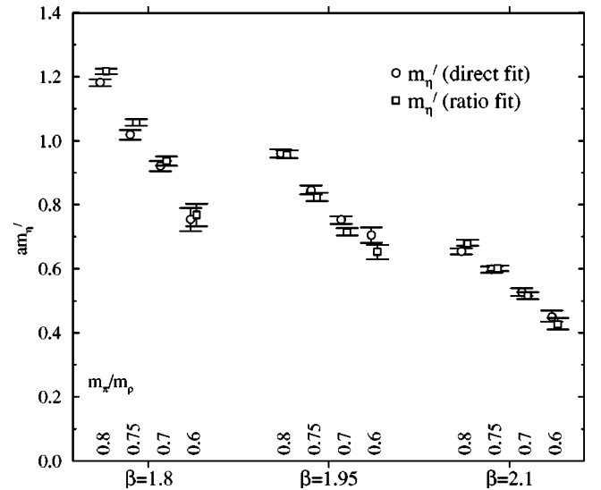
FIG. 14. Comparison of \eta' effective mass from direct and ratio fits (smeared source).
