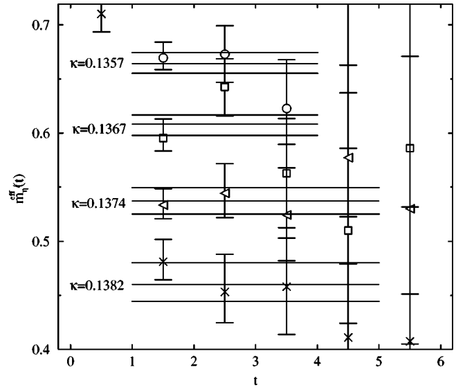
FIG. 13. \eta' effective masses m_{\eta'}^{\text{eff}}(t) from one-quark smeared sources for \beta=2.1 on a 24^3 \times 48 lattice.
