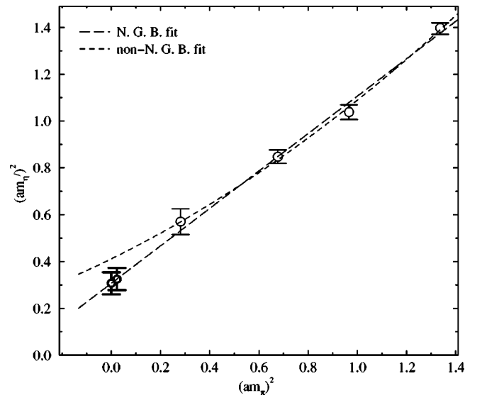
FIG. 16. Chiral extrapolation for \beta = 1.8 and smeared sources. The two extrapolated points correspond to physical and zero pion masses.
