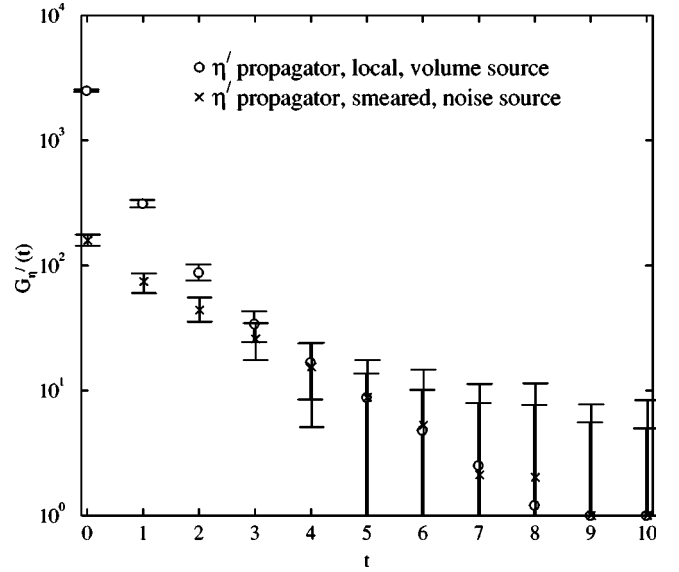
FIG. 9. Comparison of \eta' propagator for local and smeared source for \beta=2.1 and \kappa=0.1374 on a 24^3 \times 48 lattice. The local source propagator has been normalized to be coincident with the smeared source propagator at t=5 .
