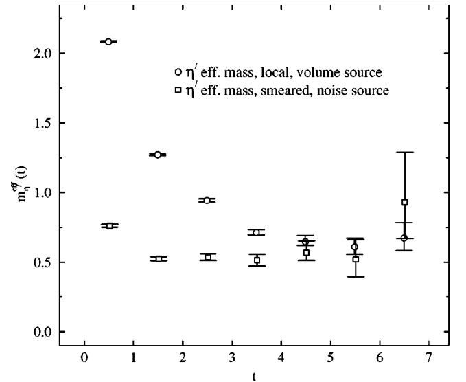
FIG. 10. Comparison of \eta' effective mass for local and smeared sources for \beta=2.1 and \kappa=0.1374 on a 24^3 \times 48 lattice.
