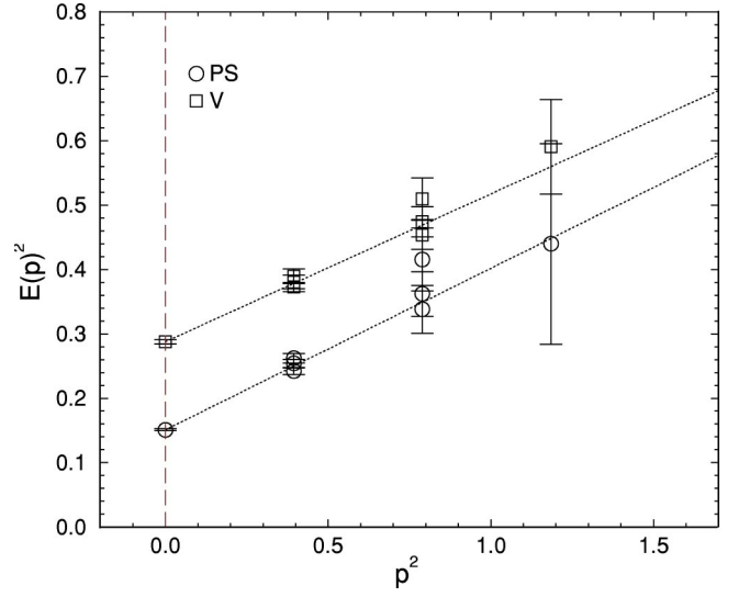
FIG. 4. Sample results for the dispersion relation of pseudoscalar and vector mesons at \beta=2.0 , \kappa=0.1244 , and (\gamma_G, \gamma_{F u_s})=(1.85, 1.60) . Dotted lines show fit results from \vec{n}=(0,0,0) and (1,0,0) .
