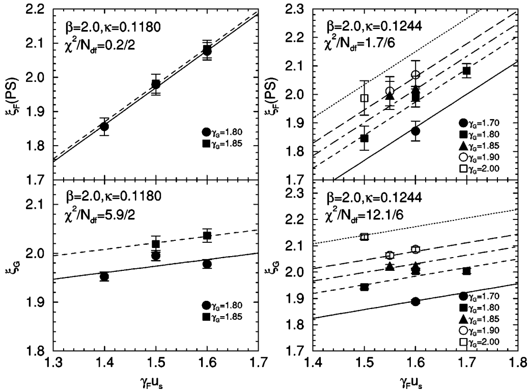
FIG. 8. The same as Fig. 6 but at \beta=2.0 .
