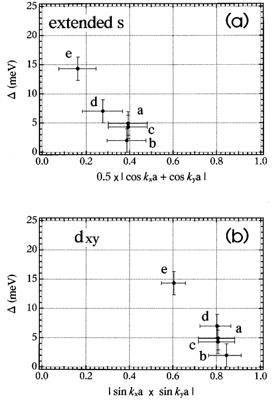
FIG. 3. The observed superconducting gap value ( \Delta ) plotted with respect to (a) the gap function of an extended s wave defined as 0.5|\cos k_x a + \cos k_y a| and (b) that of a d_{xy} wave defined as |\sin k_x a \sin k_y a| . Bars on the experimental points ( a-e ) show experimental errors due to the finite energy and angular resolutions. In either case, the experimental points are not on a straight line crossing the origin.
