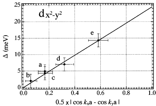
FIG. 2. The observed superconducting gap value ( \Delta ) plotted with respect to the gap function of the d_{x^2-y^2} wave defined as 0.5|\cos k_x a - \cos k_y a| . Bars on the experimental points ( a-e ) show experimental errors due to the finite energy and angular resolutions. Note that the experimental points are on or very close to a straight line which crosses the origin of the coordinate axes.
