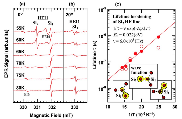
FIG. 3. (Color online) Thermally activated reorientation effect of V_{\text{C}}^- . (a) EPR spectra just for 0^\circ ( \mathbf{B} \parallel \mathbf{c} ) show the motional narrowing of the \text{Si}_1 HF line but the lifetime broadening of the \text{Si}_2 HF line. (b) Off-angle ( 20^\circ ) spectra demonstrate that the \text{Si}_1 HF structure is averaged into a single line due to the motional narrowing effect. (c) Temperature dependence of the reorientation lifetime estimated by the lifetime broadening of the \text{Si}_2 HF structure. Solid and open circles were obtained for high-field- and low-field-side \text{Si}_2 HF lines. The insets schematically show the reorientation of the defect in the (0001) plane.
