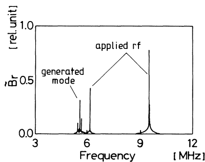
FIG. 2. Frequency spectrum of the magnetic probe signal.
