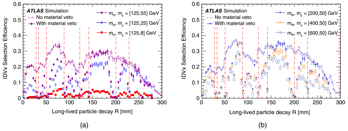
FIG. 3. IDVx selection efficiency as a function of the radial decay position for several (a) 125 GeV H \rightarrow ss and (b) \Phi \rightarrow ss mass points with m_s = 50 GeV. The dashed vertical red lines indicate the main radial material layers in the inner detector that are included in the material veto. In each figure, the IDVx selection efficiency for one signal MC sample is shown before and after the requirement of the material veto to demonstrate the impact it has on the IDVx selection efficiency.
