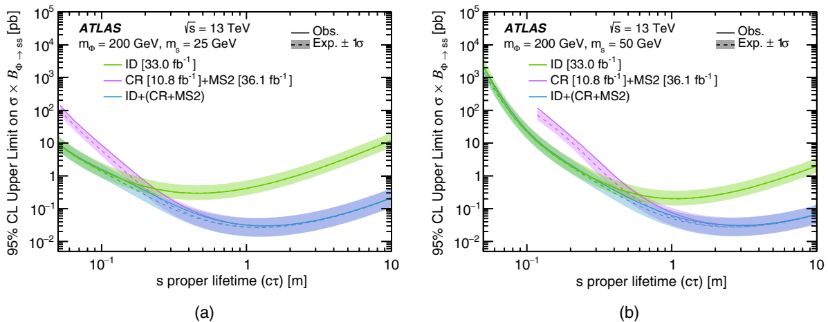
FIG. 6. Combined limits from this analysis (ID) and the CR and MS analyses for benchmark models with m_{\Phi} = 200 GeV decaying into (a) 25 and (b) 50 GeV mass scalars. The expected limit is shown as a dashed line with shading for the \pm 1\sigma error band, and the observed limit is shown with a solid line.
