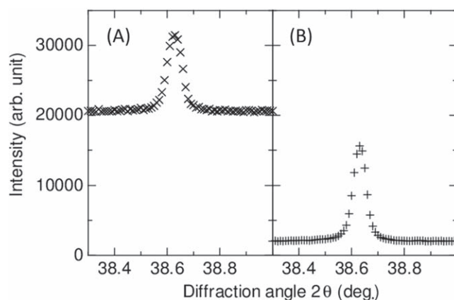
Figure 1. Plots of 620 reflection (A) for normal measurement and (B) using copper and nickel foils. The foils reduce fluorescence and characteristic x-ray intensities from molybdenum.
