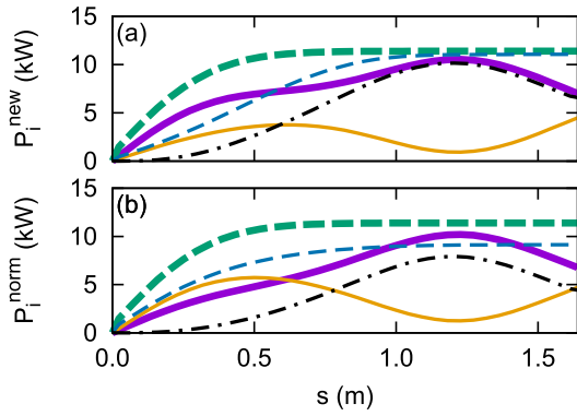
Fig. 4 Power fluxes, P_{i,\perp}^{\text{tot}} (thick solid), P_{i,\parallel}^{\text{tot}} (thin solid), P_{i,\perp}^{\text{Q}} (thick broken), P_{i,\text{rx}}^{\perp\rightarrow\parallel} (thin broken) and P_{i,\text{mirr}}^{\parallel\rightarrow\perp} (thin chain lines), with (a) the new q_{i,\perp} model and (b) the normal one.
