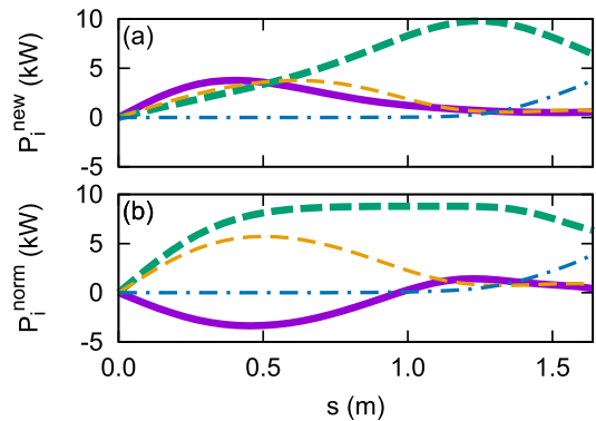
Fig. 3 Power fluxes, P_{i,\perp}^{\text{cond}} (thick solid), P_{i,\perp}^{\text{conv}} (thick broken), P_{i,\parallel}^{\text{conv,int}} (thin broken) and P_{i,\parallel}^{\text{conv,flow}} (thin chain lines), with (a) the new q_{i,\perp} model and (b) the normal one.
