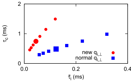
Fig. 5 Particle confinement time \tau_c as a function of \bar{\tau}_i ; the new q_{i,\perp} model (circles) and the normal one (squares). The larger symbols represent the cases with \alpha_\tau = 1 .
