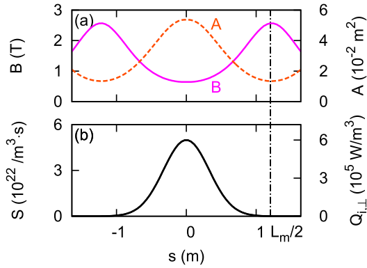
Fig. 1 Parallel-to- B profiles of (a) B (solid line), A (broken line), (b) S and Q_{i,\perp} . The vertical chain line represents the position of the local maximum of B ( s = L_m/2 ).
