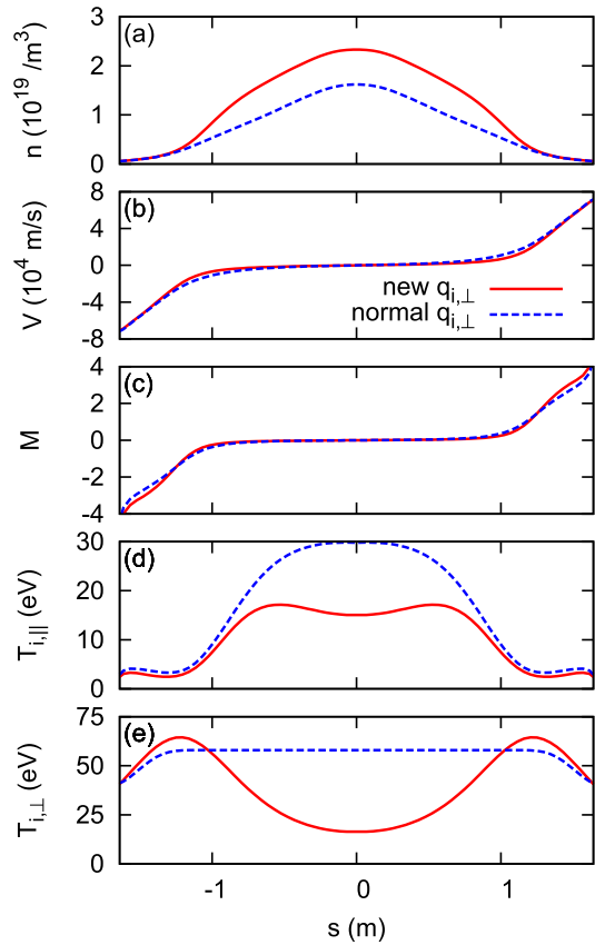
Fig. 2 Parallel-to- B profiles of plasma parameters between the new q_{i,\perp} model (solid lines) and the normal one (broken lines); (a) n , (b) V , (c) M (d) T_{i,\parallel} and (e) T_{i,\perp} .
