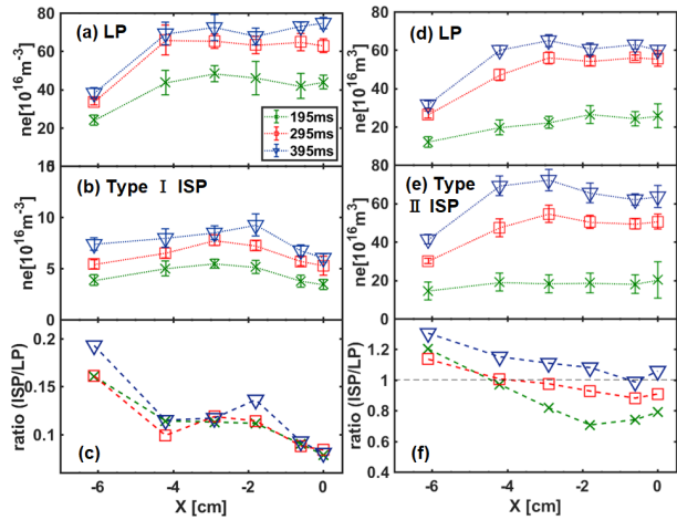
Fig. 3 X profile of the electron density measured by (a) LP and (b) Type-I ISP guard electrode. (c) Ratio of electron density measured using Type-I ISP and LP. (d), (e), and (f) show results of Type-II ISP, and LP, comparatively.
