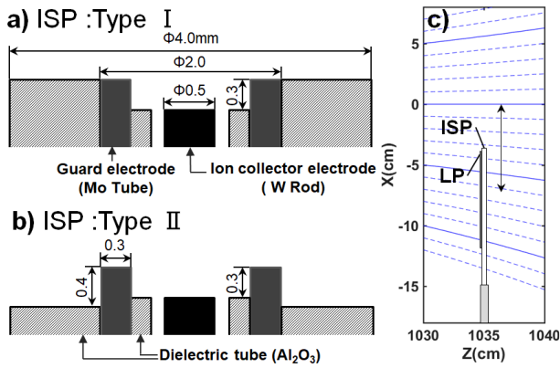
Fig. 1 (a) Type-I ISP head structure: guard electrode was aligned with the outer dielectric tube. (b) Type-II ISP head structure: guard electrode protruded 0.4 mm from the outer dielectric tube. (c) Magnetic field lines in X - and Z -directions around the ISP measurement position, at the inlet of the D-module of GAMMA 10/PDX.
