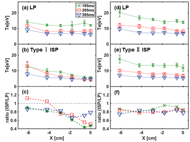
Fig. 2 X profile of the electron temperature using (a) LP and (b) Type-I ISP guard electrode. (c) Ratio of electron temperatures measured using Type-I ISP and LP. (d), (e), and (f) show the results of Type-II ISP and LP.
