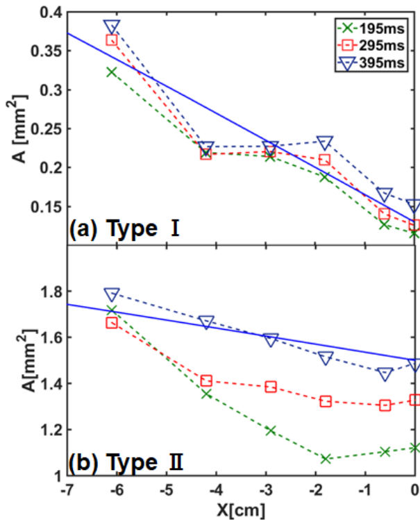
Fig. 4 Evaluation of effective collection area using Eq. (2) for (a) Type-I ISP and (b) the Type-II ISP. Blue solid lines indicate the incident area of the magnetic field lines.
