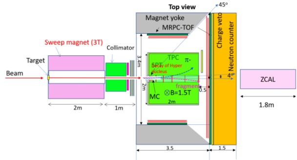
Fig. 6. The top view of the hypernuclear spectrometer.
