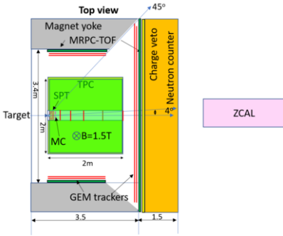
Fig. 1. The top view of the hadron spectrometer.
