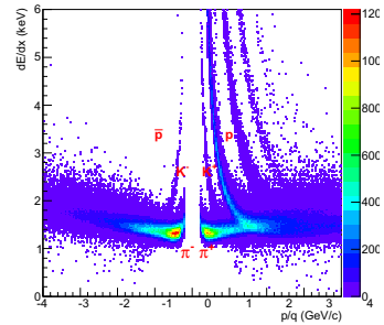
Fig. 4. dE/dx in TPC vs rigidity (GeV/c).
