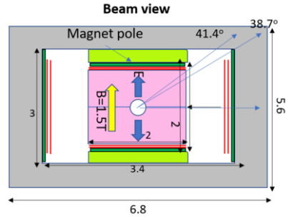
Fig. 2. The beam view of the hadron spectrometer.
