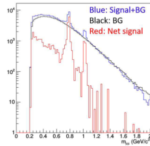
Fig. 8. The fully simulated and reconstructed dimuon spectrum.
