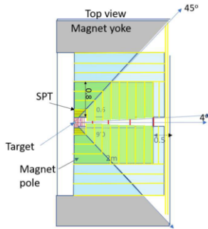
Fig. 5. The top view of the dimuon spectrometer.
