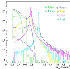
Fig. 7. The cocktail spectrum of dimuons.
