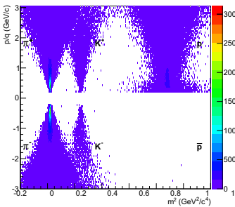
Fig. 3. Rigidity ( p/q ) (GeV/c) vs mass-squared ( \text{GeV}^2/c^4 ).
