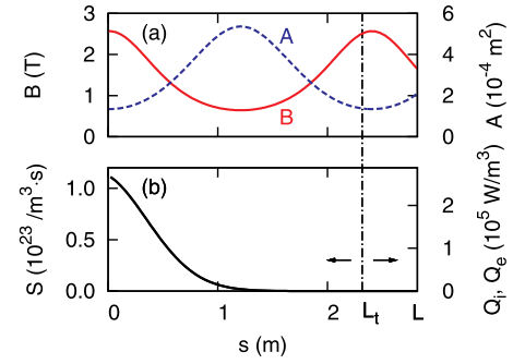
Fig. 1. Calculation conditions used in this study; parallel-to- B profiles of (a) the magnetic field strength B (solid line), the cross-sectional area of the flux tube A (broken line) and (b) source terms. The vertical chain line represents the target position.
