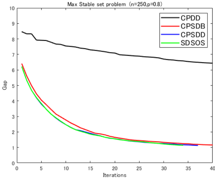
Figure 1: Relation between the number of iterations and the gap
