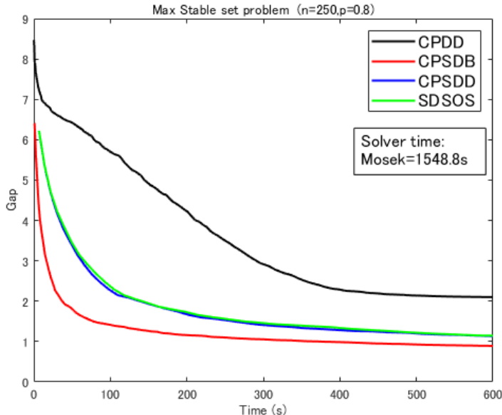
Figure 2: Relation between the computational time (s) and the gap
