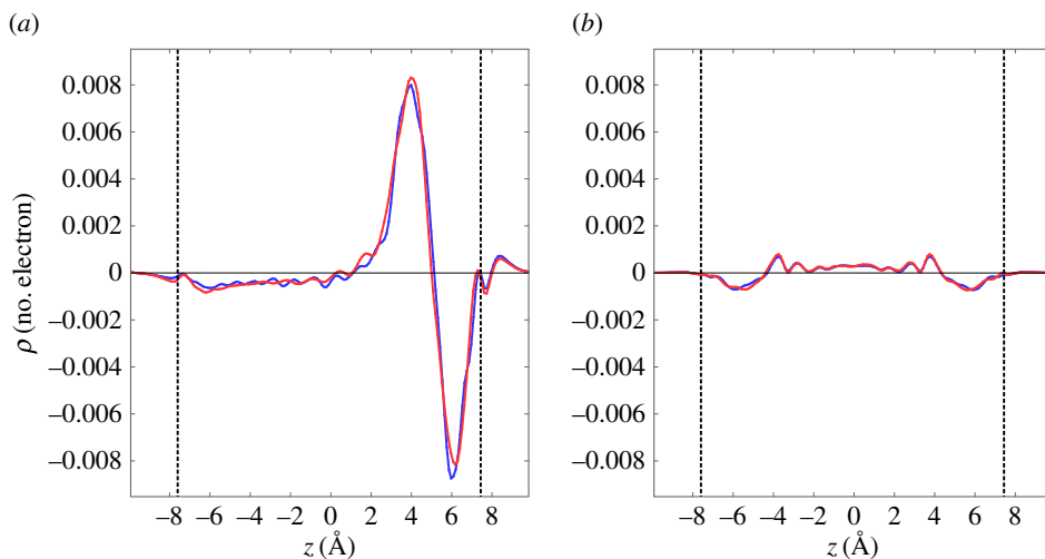
Figure 4. Plane averaged charge redistribution along the z direction inside a CNT upon perylene encapsulation with molecular tilt angles of (a) 0^\circ and (b) 70^\circ with respect to the C_2 axis parallel to the zigzag edges of perylene. Blue and red lines denote the electron density of (11,11) and (19,0)CNTs, respectively, encapsulating perylene. The vertical dashed lines indicate the position of the CNT walls.
