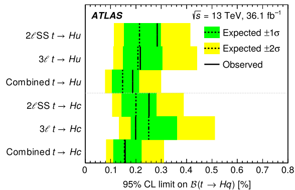
FIG. 3. Observed and expected 95% C.L. upper limits on B(t \rightarrow Hu) and B(t \rightarrow Hc) . In each case, the other FCNC decay is assumed to have zero branching fraction. The individual results from each signal category are shown as well as the combination.
