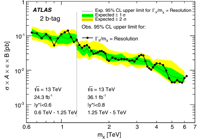
FIG. 9. Observed (filled circles) and expected (dotted line) 95% credibility-level upper limits on \sigma \times A \times \epsilon \times \mathcal{B}(X \rightarrow b\bar{b}) , including kinematic acceptance and b -tagging efficiencies, for resonances with intrinsic width smaller than the detector resolution. The width of the Gaussian reconstructed shape is dominated by the dijet mass resolution. The plot shows the limits obtained from the combined low- and high-mass (separated by the vertical dotted line) two b -tags selection.
