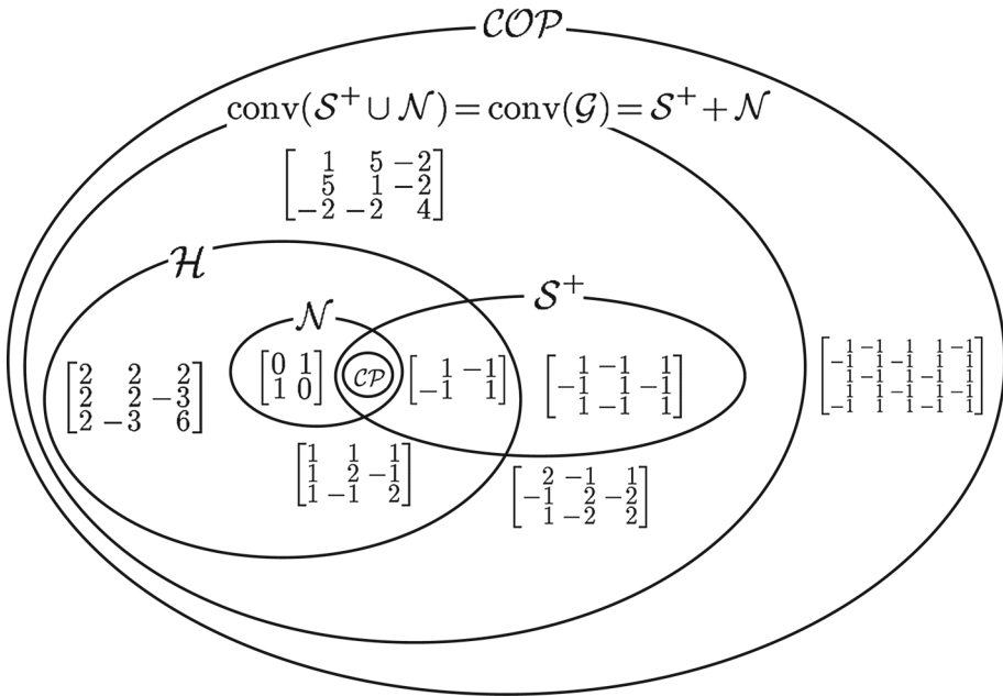
Fig. 2 Examples of inclusion relations among the subcones of S_n^+ + \mathcal{N}_n II
