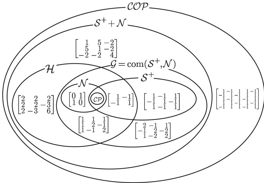
Fig. 1 Examples of inclusion relations among the subcones of S_n^+ + \mathcal{N}_n
