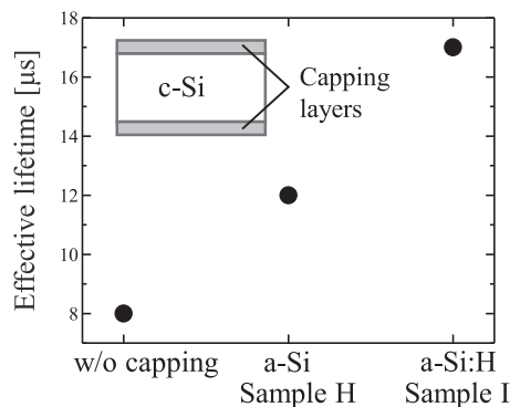
FIG. 3. Effective carrier lifetimes of c-Si(111) substrate ( \rho = 6\text{--}9 \Omega\text{cm} ), and the c-Si(111) substrates covered on both front and back mirror surfaces with approximately 20 nm-thick pure a-Si (sample H) and a-Si:H layers (sample I). The density of photoexcited electron and hole pairs was approximately 10^{15} \text{ cm}^{-3} .
