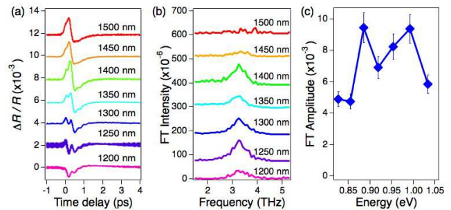
FIG. 5. (a) Time-resolved reflectivity changes for crystalline GST225 film with fixed pump (800 nm) and various probe wavelengths. (b) FT spectra of (a) are shown. We omit the FT spectrum at 1550 nm due to larger noise, making unable to compare with others. (c) The peak FT amplitude of the A_1 mode obtained from (b) plotted as a function of the probe photon energy. The amplitude becomes larger as the photon energy increases and at 1.0 eV ( \approx 1250 \text{ nm} ), it is about \sim 200\% larger than that at 0.83 eV ( \approx 1500 \text{ nm} ).
