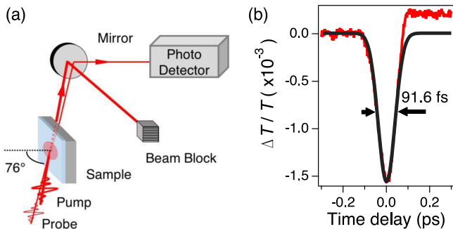
FIG. 1. (a) Experimental configuration around the sample (GST225). The angle of incidence has been adjusted to the Brewster angle ( \approx 76^\circ ) to efficiently excite the sample. (b) Time-resolved transmission change in the Si(111) substrate (red) and its Gaussian fit (black). Transient reduction in the transmission is caused by two photon absorption (TPA), whose FWHM is estimated to \approx 91.6 fs by the Gaussian fit.
