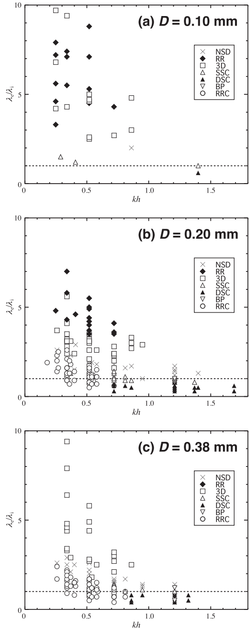
Fig. 2 The relationship between kh and \lambda_e/\lambda_i for the occurrence of distinctive transient ripples: (a) D = 0.10 mm, (b) D = 0.20 mm, and (c) D = 0.38 mm.
