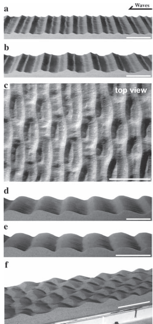
Fig. 1 Characteristic transient ripples, which ephemerally occur during ripple modification: (a) ripples with a single secondary crest (SSC), (b) those with double secondary crests (DSC), (c) barrel-type ripples (BR), (d, e) round-crested ripples (RC), and (f) rhombic-type ripples (RR). Scale bar shows 10 cm.
