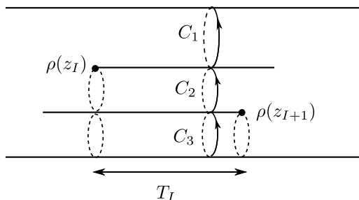
Figure 5. C_1, C_2, C_3 are the contours corresponding to the variation T_I \rightarrow T_I + \delta T_I .
