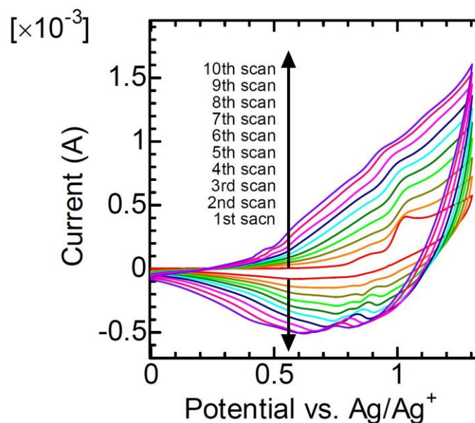
FIGURE 2 Cyclic voltammetry (CV) result in 10 scans versus Ag/Ag + reference electrode during polymerization under circularly polarized light. Polymerization under pulse L-CPL at 532 nm.
