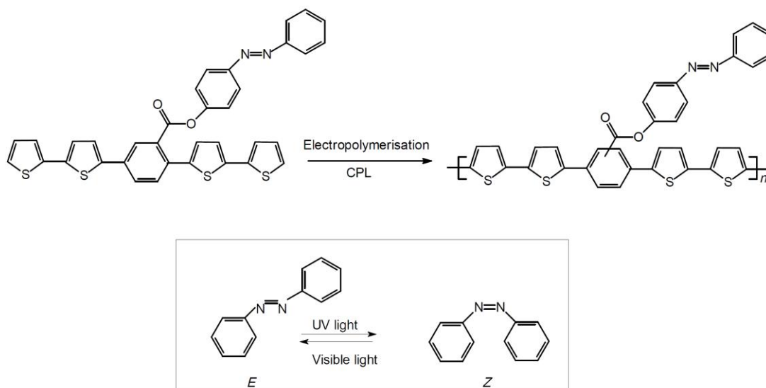
SCHEME 1 Electropolymerization under L-CPL or R-CPL. CPL = circular polarized light.
