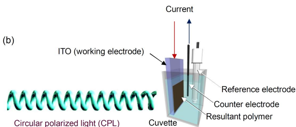
FIGURE 1 (a): Electrochemical polymerization under irradiation by circular polarized laser light. (b): Set up of electrochemical polymerization cell.
