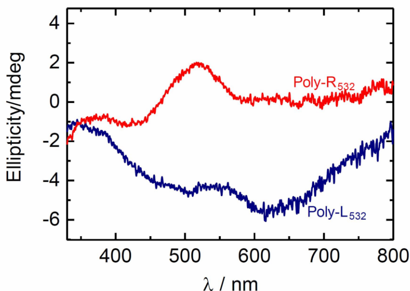
FIGURE 3 Circular dichroism (CD) absorption spectra of the polymers. Poly-R 532 : polymer obtained under right circular polarized light (R-CPL). Poly-L 532 : polymer obtained under left circular polarized light (L-CPL).
