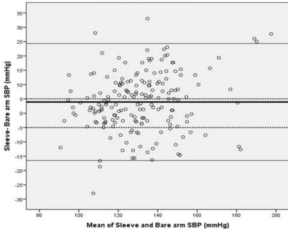
Bland-Altman plot of differences in systolic blood pressure readings between bare arm and sleeved arm
