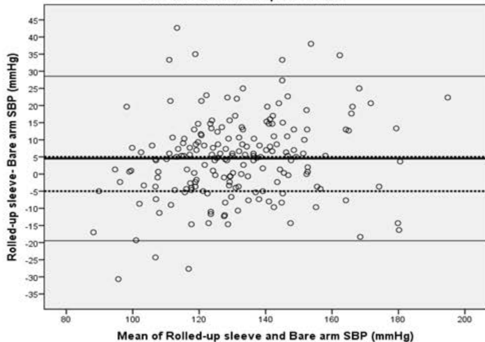
Bland-Altman plot of differences in systolic blood pressure readings between bare arm and rolled-up sleeve arm
