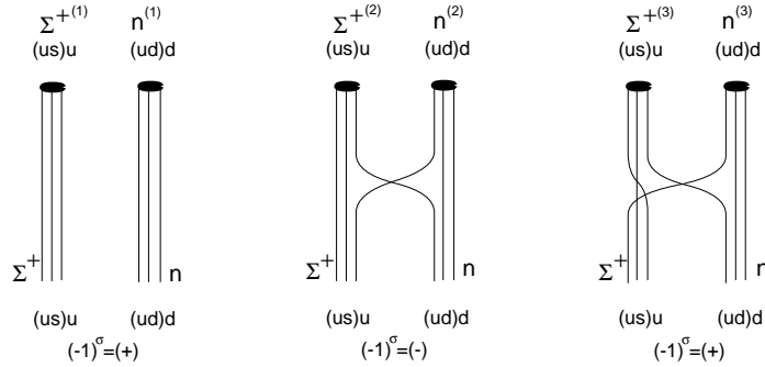
Figure A.3: Diagrammatic representation of the four-point correlation function \langle \Sigma^+ n \overline{\Sigma^+ n} \rangle . Three diagrams correspond to the three terms in Eq. (A.3). The parity of each permutation is also shown as (-1)^\sigma .
