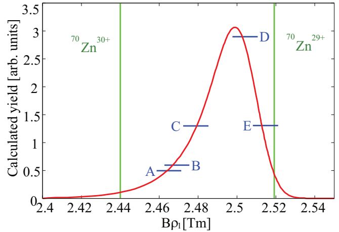
FIG. 1. Calculated momentum distribution of ^{69}\text{Cu} by the LISE++ program [20]. A ( -1.30\% ), B ( -1.19\% ), C ( -0.80\% ), D ( +0.16\% ), and E ( +0.75\% ) correspond to the different momentum selections. The values in the brackets correspond to the central values of each momentum selection with respect to the center of the momentum distribution. The width of the momentum selection was 0.5\% in each of the cases.
