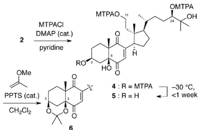
Scheme 1. Preparation of the MTPA esters of aplysiaseosterol B ( 2 ) and their degradation.
