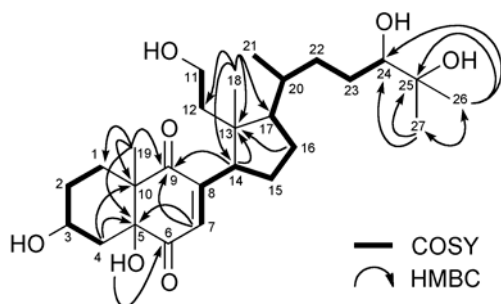
Fig. 2. Planar structure of aplysiaseosterols B ( 2 ) and C ( 3 ) determined by 2D-NMR analysis (arrows, selected HMBC correlations).
