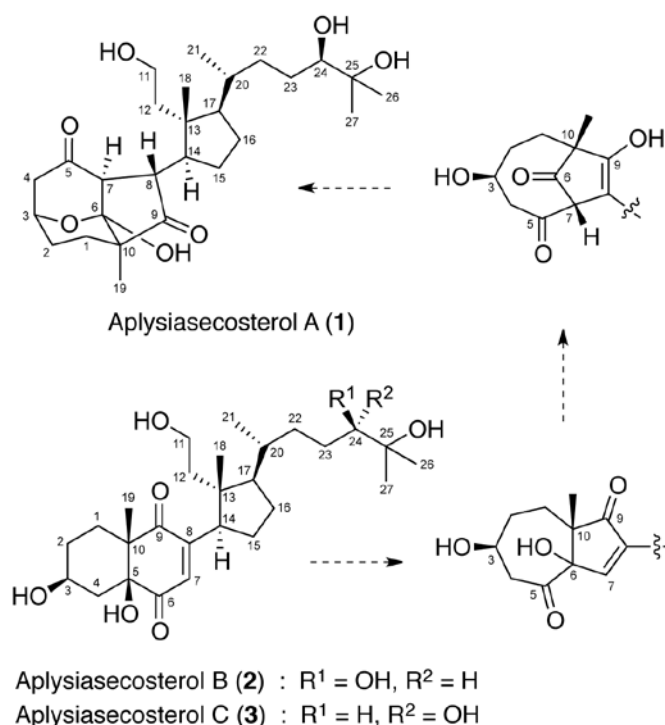
Fig. 1. Structures of aplysiasecosterols A–C and their proposed biosynthetic intermediates.
