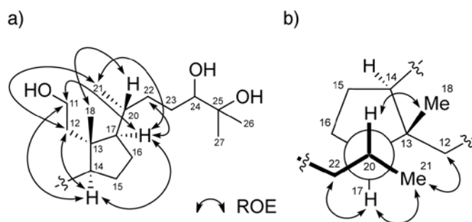
Fig. 3. (a) Relative stereochemistry around the cyclopentane rings of aplysiaseosterols B ( 2 ) and C ( 3 ) determined from the ROESY spectrum. (b) A Newman projection with a view along the C20–C17 bond.
