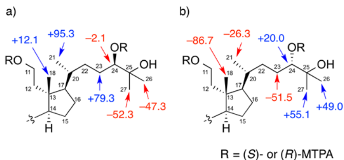
Fig. 4. \Delta\delta values ( \delta_S - \delta_R ) for the 11,24-bis-MTPA esters 5 prepared from (a) aplysiasecosterol B ( 2 ) and (b) aplysiasecosterol C ( 3 ) in Hz (600 MHz, CD 3 OD).
