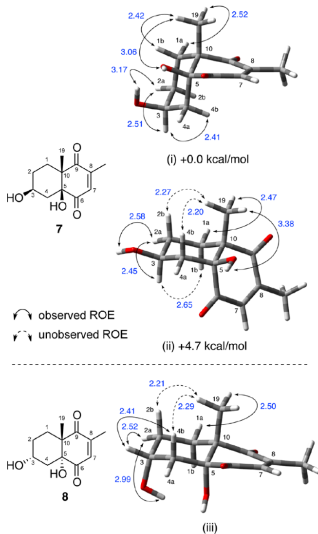
Fig. 5. Structures of the cis - and trans -fused 1,4-quinones 7 and 8 and their optimized structures at the B3LYP/6-31G+(d,p) level of theory in implicit solvation model (CPCM, CHCl 3 ). The relative energy of conformers (i) and (ii) is shown below. Observed and unobserved ROEs in aplysiasecosterol B ( 2 ) are shown as solid and dashed arrows, respectively. Values in blue represent the calculated distances between two selected protons in Å.
