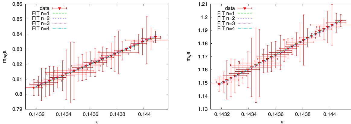
FIG. 12 (color online). The \kappa dependence of m_{PSa} (left panel) and m_{Va} (right panel) on the line of constant physics at m_{PS}/m_V = 0.70 . Results of n th order polynomial fits are also shown.
