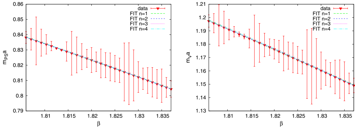
FIG. 10 (color online). The \beta dependence of m_{PSa} (left panel) and m_{Va} (right panel) on the line of constant physics at m_{PS}/m_V = 0.70 . Results of n th order polynomial fits are also shown.
