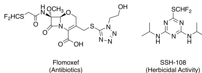
Figure 2. Useful difluoromethylsulfanylated compounds.
