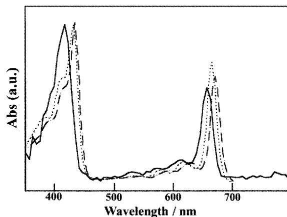
Fig. 5 Absorption spectra in 20-Cl-Chl a (---) and authentic Chl a (···) in benzene (Kobayashi et al. 1988), and a new pigment (—) in an HPLC eluent.
