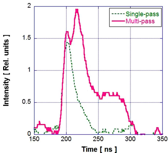
FIG. 3. Single (green dotted line) and multi-pass (red line) TS signals.
