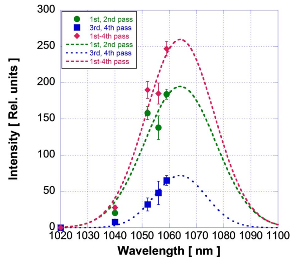
FIG. 4. TS spectra of the multi-pass configuration.
