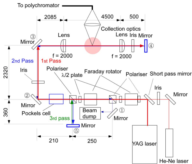
FIG. 1. Schematic of the multi-pass TS system.
