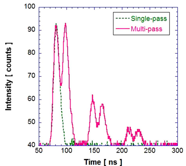
FIG. 2. Single (green dotted line) and multi-pass (red line) Raman scattering signals of CH. 1.
