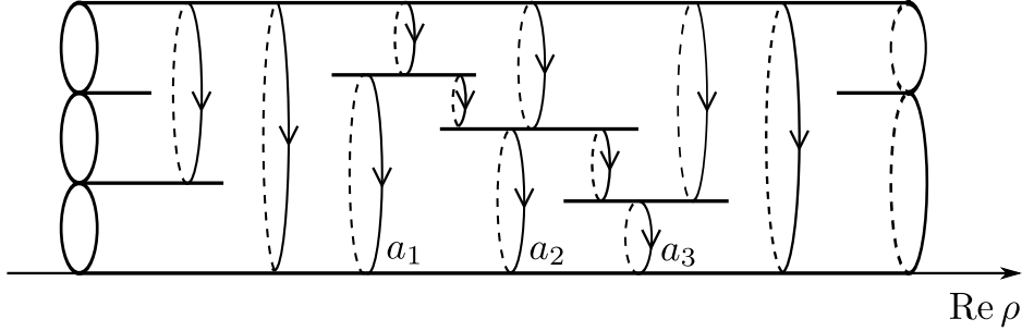
Figure 1: A string diagram with 3 incoming, 2 outgoing strings and 3 loops. The cycles \mathcal{C}_{\mathcal{I}} going around the cylinders corresponding to the internal propagators are described. Among them, the cycle a_j is the a cycle for the j -th loop.
