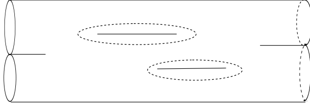
Figure 3: The cycles corresponding to the variations of the + components of the loop momenta.
