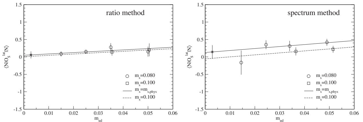
FIG. 9. Linear extrapolations of \langle N | \mathcal{O}_S^{\text{lat}} | N \rangle obtained from ratio (left panel) and spectrum (right panel) methods. Solid and dashed lines show the fit lines at m_s = m_{s,\text{phys}} and 0.100, respectively. We omit the fit line at m_s = 0.080 , which is not indistinguishable from that at m_s = m_{s,\text{phys}} in the scale of the figure. Star symbols represent \langle N | \mathcal{O}_S^{\text{lat}} | N \rangle extrapolated to the physical quark masses. Square symbols are slightly shifted in the horizontal direction for clarity.
