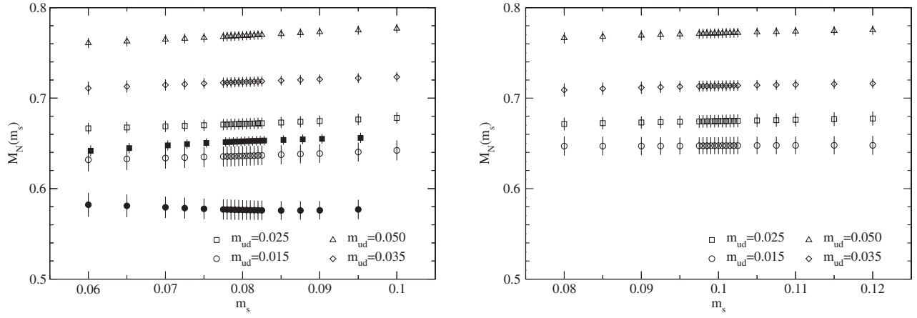
FIG. 6. Nucleon masses M_N as a function of m_s . Left and right panels show M_N obtained by reweighting from that at m_s = 0.080 and 0.100 , respectively. We plot results on the 16^3 \times 48 and 24^3 \times 48 lattices, by open and filled symbols. Filled squares are slightly shifted in the horizontal direction for clarity.
