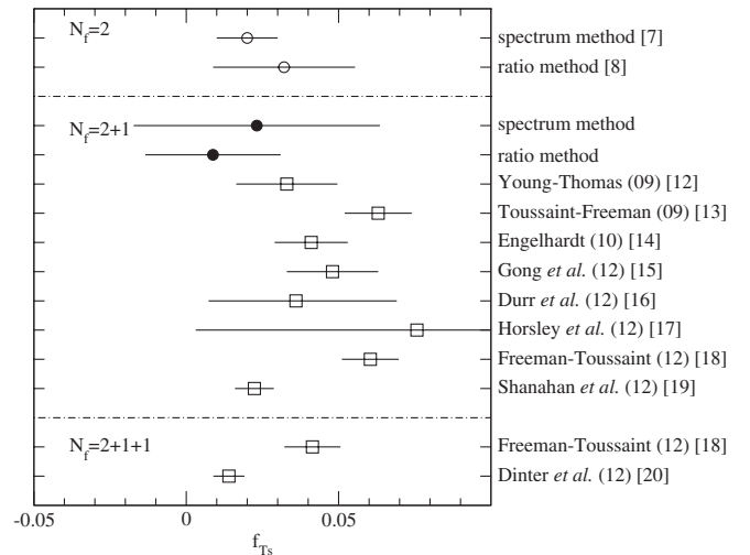
FIG. 12. Comparison of f_{T_s} with our previous studies in N_f = 2 QCD and recent studies in N_f = 2 + 1 and 2 + 1 + 1 QCD [12–20]. We convert m_s \langle N|\bar{s}s|N\rangle or \langle N|\bar{s}s|N\rangle in Refs. [13,17–19] to f_{T_s} using the experimental value of M_N and m_s obtained in Ref. [41].
