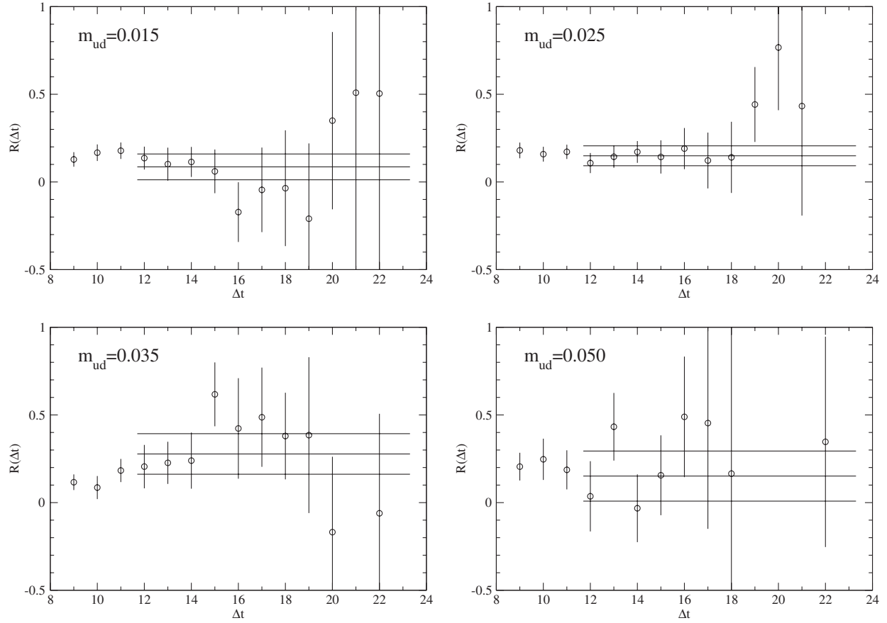
FIG. 4. Results of the constant fit to R(\Delta t, \Delta t_s) as a function of \Delta t . Four panels show results obtained at different values of m_{ud} and at m_s = 0.080 .
