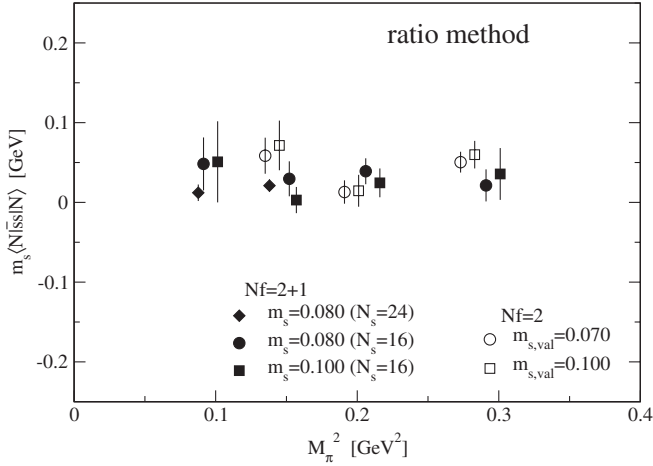
FIG. 13. A comparison of a renormalization invariant quantity m_s\langle N|\bar{s}s|N\rangle between N_f = 2 (Ref. [8], open symbols) and 2 + 1 (this study, filled symbols) QCD. We plot data from the ratio method as a function of M_\pi^2 .
