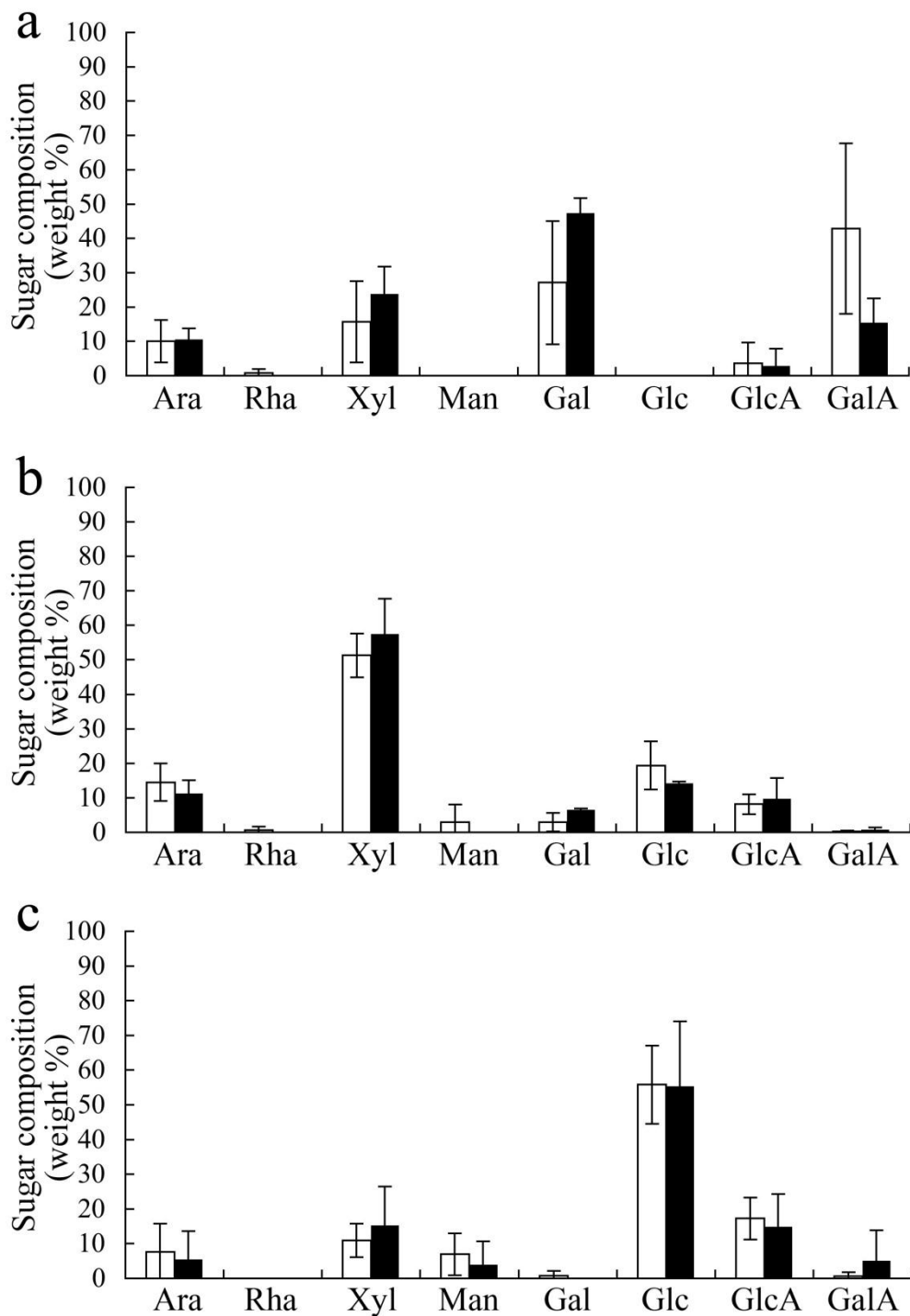
Fig. 3 Sugar composition of cell wall fractions in rice shoots grown under +Si/-Si conditions for 4 weeks. Sugar composition of 50 mM Na 2 CO 3 -soluble ( a ) and 4 M KOH-soluble ( b ) fractions, and 4 M KOH-insoluble residue ( c ) obtained from rice shoots (n = 3). Black and white bars indicate -Si and +Si conditions, respectively.
