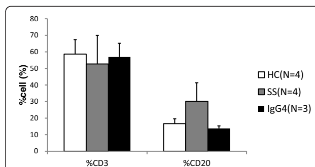
Figure 1 The cell population of CD3-positive T cells and CD20-positive B cells in peripheral blood mononuclear cells. PBMCs stained with anti-CD3 antibody and anti-CD20 antibody were analyzed and sorted with flow cytometry. HC, healthy control; SS, Sjögren syndrome; IgG4, IgG4-RD.
