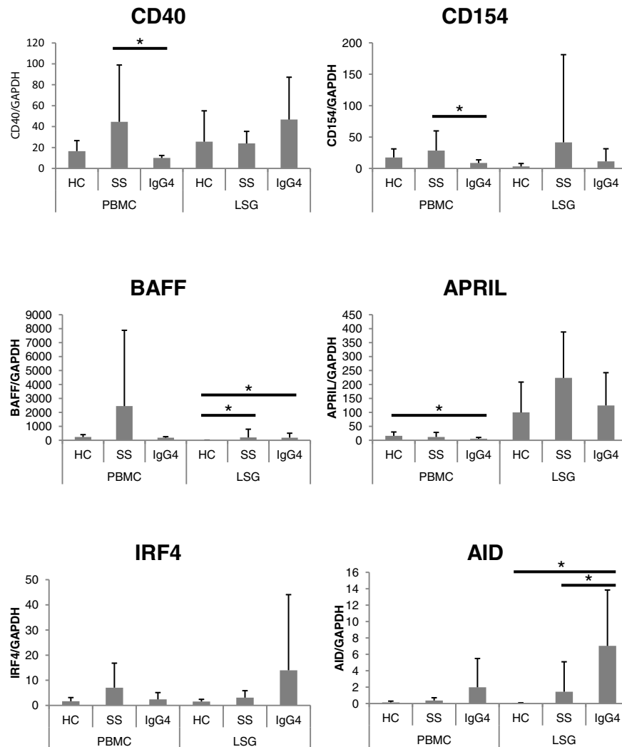
Figure 3 The mRNA expression levels of IgG4-nonspecific class switch-related molecules in PBMCs and LSGs. The displayed mRNA expression levels are relative to the mRNA level of GAPDH, representing the internal control. Data are expressed as mean \pm SD. * P < 0.05 , Mann-Whitney U -test. PBMCs, peripheral blood mononuclear cells; LSGs, labial salivary glands; HC, healthy control; SS, Sjögren syndrome; IgG4, IgG4-RD.
