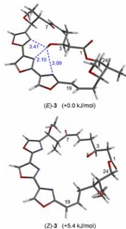
Fig. 2. Optimized structures and relative energies of 3 at the B3LYP/6-31G(d) level of theory. Values in ( E )- 3 represent the calculated distances between the C3 hydroxyl H atom and the three oxazole N atoms (Å).
