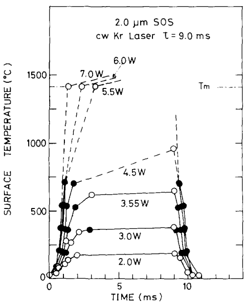
FIG. 3. Time-resolved surface Si lattice temperatures obtained from the data in Figs. 1 and 2, and others.
