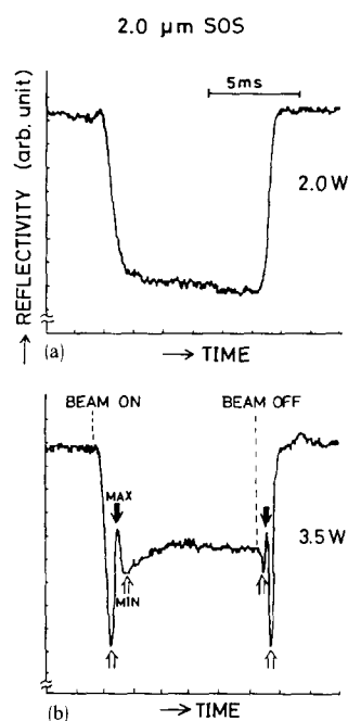
FIG. 1. Typical time-resolved optical reflectivity traces for 2.0- \mu\text{m} SOS during cw laser annealing for (a) 2-W and (b) 3.5-W laser powers, indicating no melting.
