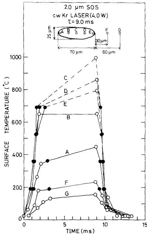
FIG. 4. Time-resolved and space-resolved surface Si lattice temperatures which are obtained from the time-resolved reflectivity traces proved at various points shown in the inset.
