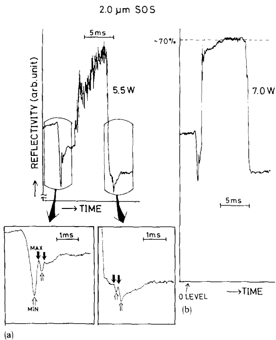
FIG. 2. Typical time-resolved optical reflectivity traces indicating Si melting. In trace (a), two expanded traces are added to show more clearly reflectivity changes around at times when the shutter is opened and closed, respectively.
