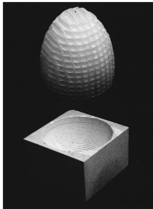
FIG. 2. Three-dimensional image of the new filter and the bolus designed for the conformal irradiation on a spherical target.
