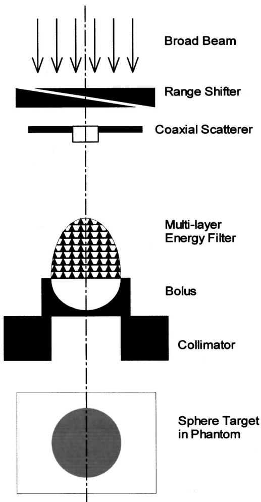
FIG. 3. Schematic drawing of the experimental setup for three-dimensional conformal irradiation.
