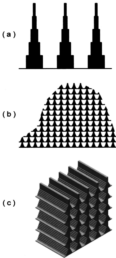
FIG. 1. Schematic drawing of energy filters. (a) Traditional ridge filter. (b) Multilayer filter. (c) Three-dimensional image of part of the new filter.
