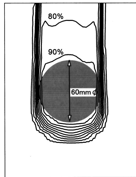
FIG. 4. Experimental result of the dose distribution measured by a stack of imaging plates. Data are interpolated from the three-dimensional data on a plane along the beam axis.
