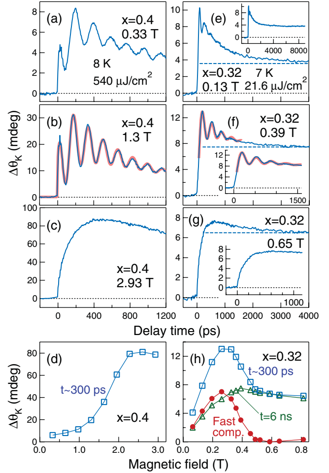
FIG. 2 (color). Time evolution of \Delta\theta_K and the field dependence. (a)–(c) \Delta\theta_K(t) for x = 0.4 at temperature T = 8 K. The excitation density is D_e = 540 \mu\text{J}/\text{cm}^2 [22]. (d) Field dependence of the \Delta\theta_K at t \sim 300 ps for x = 0.4 . (e)–(g) \Delta\theta_K(t) for x = 0.32 at T = 7 K, D_e = 21.6 \mu\text{J}/\text{cm}^2 . Horizontal broken lines represent the \Delta\theta_K at 6 ns (the magnitude of the slow decay component). The red curves in (b) and (f) are the fitting ones [19]. (h) Field dependence of the \Delta\theta_K for x = 0.32 at t \sim 300 ps (squares) and t = 6 ns (triangles). The intensity of the fast component (closed circles) is obtained by \Delta\theta_K(300 \text{ ps}) - \Delta\theta_K(6 \text{ ns}) . The solid lines in (d) and (h) are merely guides to the eyes.
