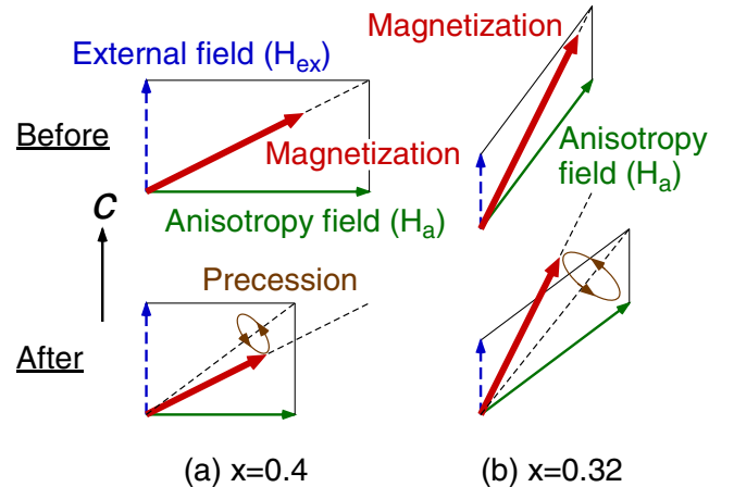
FIG. 4 (color online). Excitation process of magnetization precession for (a) x = 0.4 and (b) x = 0.32 . Thick arrows are the magnetization. In both the cases, external field (broken arrows) is along the c axis. Anisotropy field (thin arrows) is parallel to the ab plane for x = 0.4 . It should be parallel to the c axis for x = 0.32 in the bulk, but is assumed to be fractionally tilting due to the demagnetizing field at the sample surface [20].
