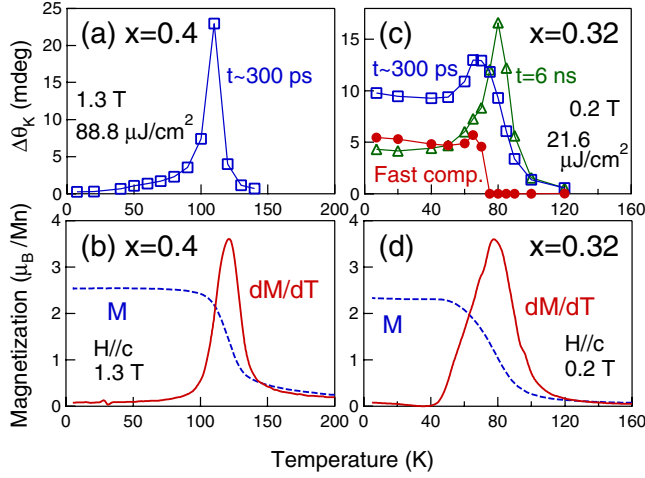
FIG. 3 (color online). Temperature dependence of \Delta\theta_K and magnetization. (a) \Delta\theta_K at t \sim 300 ps for x = 0.4 ( H = 1.3 T, D_e = 88.8 \mu\text{J}/\text{cm}^2 ). (b) Magnetization (broken line) and its first derivative (solid line) for x = 0.4 in the same field as (a). (c) \Delta\theta_K for x = 0.32 ( H = 0.2 T, D_e = 21.6 \mu\text{J}/\text{cm}^2 ) at t \sim 300 ps (squares, obtained by averaging) and 6 ns (triangles). The fast component (closed circles) is derived by \Delta\theta_K(300 \text{ ps}) - \Delta\theta_K(6 \text{ ns}) [23]. (d) Magnetization and its first derivative for x = 0.32 in the same field as (c).
