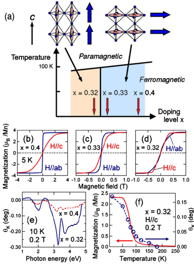
FIG. 1 (color online). Magnetic and magneto-optical properties of \text{La}_{2-2x}\text{Sr}_{1+2x}\text{Mn}_2\text{O}_7 . (a) Schematic phase diagram. Ferromagnetic spin order (thick arrows) is drawn in the upper part with \text{MnO}_6 octahedra and the e_g electron orbital occupancy (left: d_{3z^2-r^2} , right: d_{x^2-y^2} ). (b)–(d) Magnetization curves at 5 K for x = 0.4, 0.33, and 0.32 . (e) Magneto-optical Kerr rotation \theta_K spectra at 10 K in the field of 0.2 T along the c axis. They are taken with reflection from the ab surfaces of the samples at x = 0.32 (solid) and 0.4 (broken line) by the optical retardation modulation method [21]. (f) Temperature dependence of \theta_K at 3.1 eV (circles) and magnetization (solid line) for x = 0.32 ( H \parallel c, 0.2 T). The broken line in (f) is merely a guide to the eyes.
