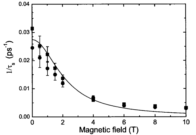
FIG. 4. Magnetic field dependence of the spin relaxation rate. The experimental values from time-resolved PL (circles) and the estimated values from steady-state PL spectra (squares) are shown together for comparison. The solid line is the theoretical fitting according to Eq. (2).
