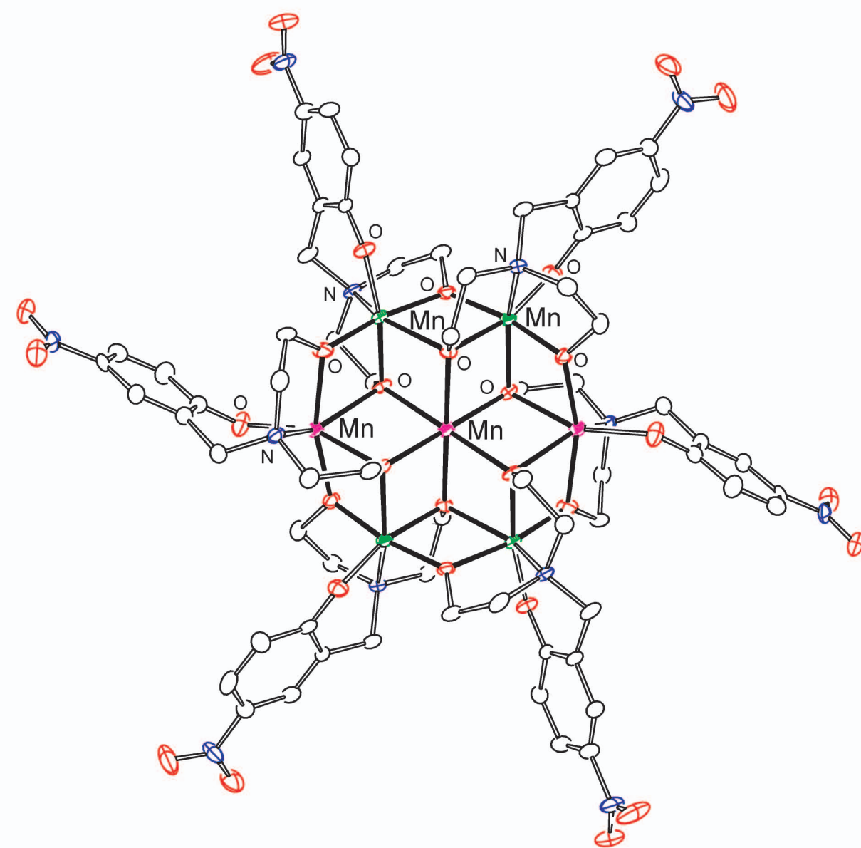
Wheel SMM of [\text{Mn}^{\text{II}}_3\text{Mn}^{\text{III}}_4]
